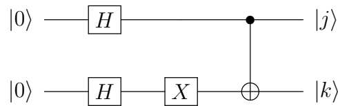
Figure 5.9: Sample quantum algorithm
