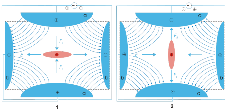
Figure 3.2: A schematic drawing of the Paul Trap
