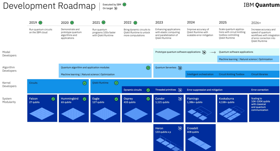
Figure 7.1: IBM's Quantum Development Roadmap
