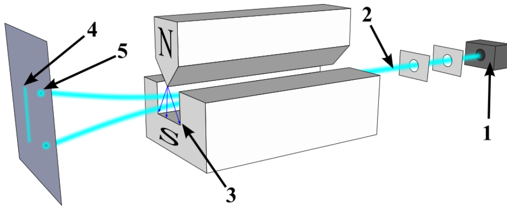
Figure 2.2: Stern-Gerlach Experiment
