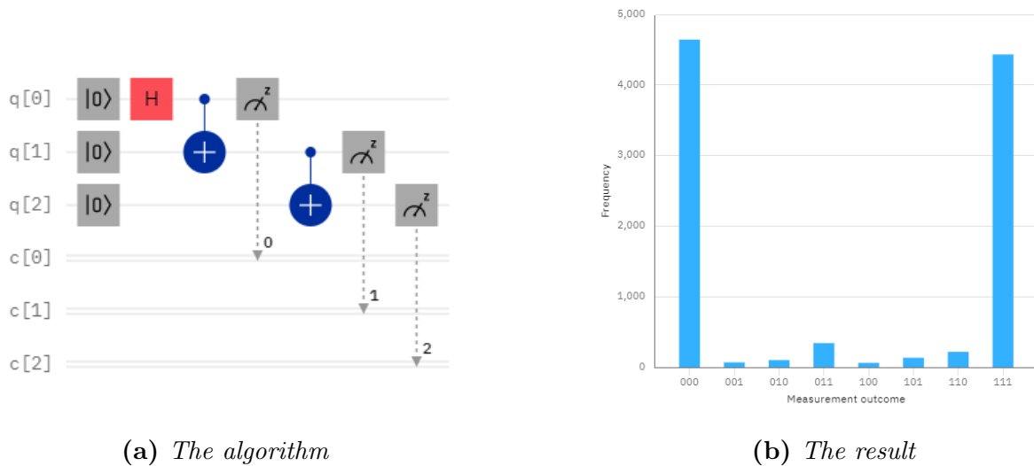
Figure 6.5: Circuit to create the GHZ state with 3 qubits
