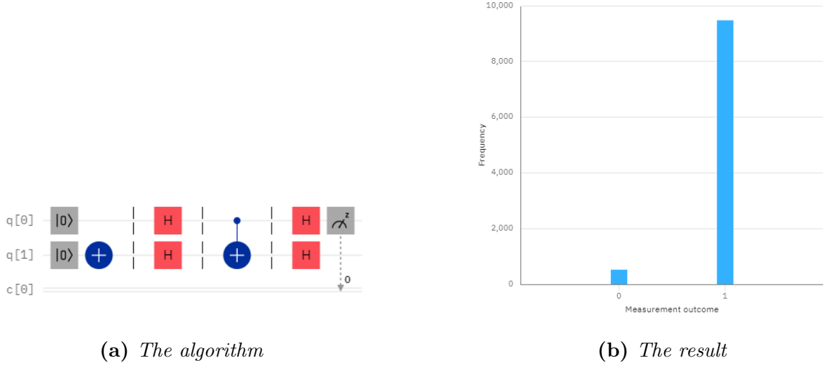
Figure 6.3: The Deutsch f_1 algorithm
