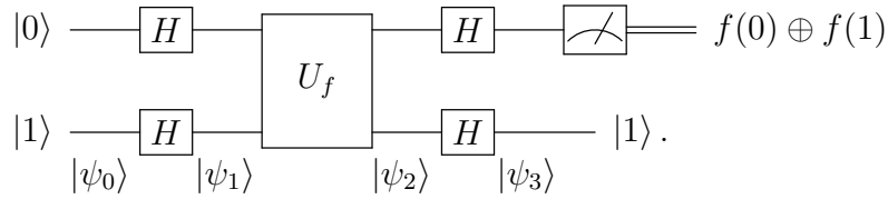
Figure 6.1: Deutsch Algorithm
