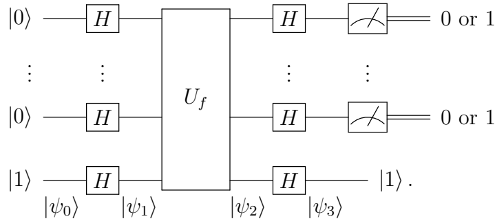
Figure 6.4: Deutsch-Jozsa algorithm
