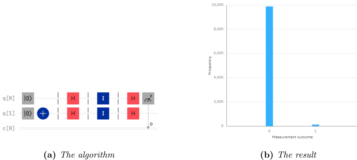
Figure 6.2: The Deutsch f_0 algorithm
