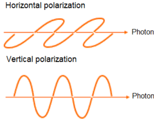
Figure 3.1: States of a qubit realized with photons
