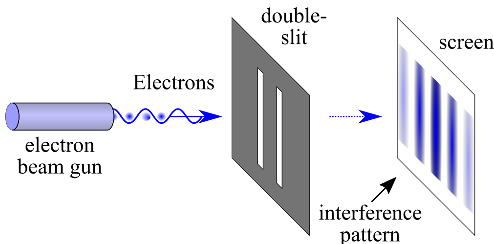
Figure 2.1: Double slit experiment
